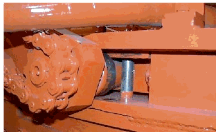
Lower Drillhead Until Roller Assembly's Resting Against Pin
